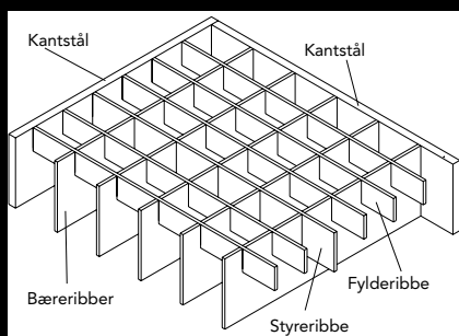
Skraberist, maske 32x22 mm.
